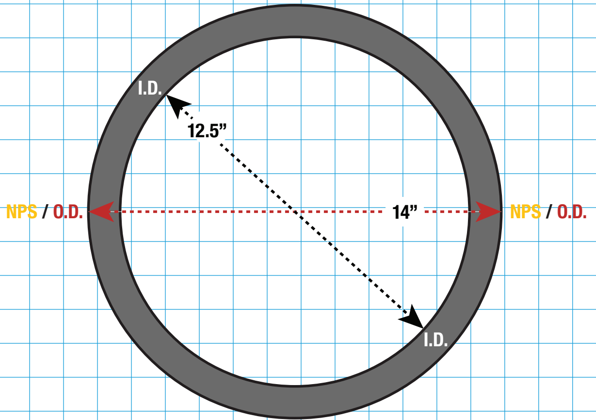
14" SCHEDULE 80 PIPE SIZE & THICKNESS
