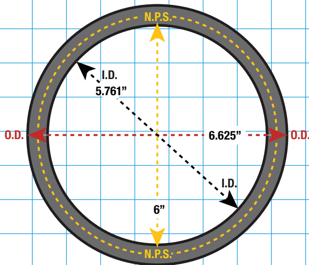
6" SCHEDULE 80 PIPE SIZE & THICKNESS
