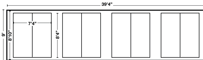
FRONT SIDE VIEW (SHOWN WITH DOUBLE CARGO DOORS - REAR SIDE HAS 4 ROLL UP DOORS)
