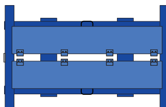
EZ Lock Blind Flange Rack®
