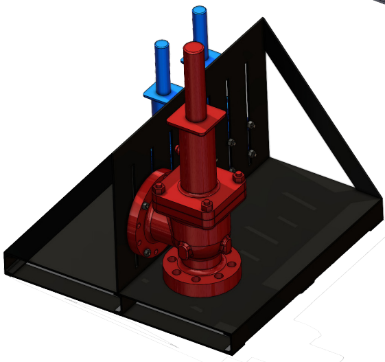
PSV-610 Shown with 6" & 10" Valves Mounted to Rack Frame
