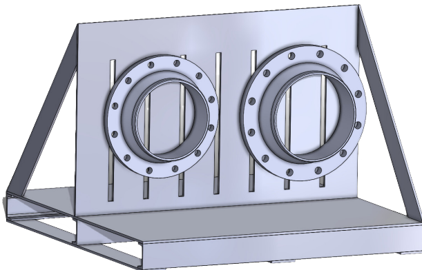
PSV-1216 (12" - 16") Flanges & Valves
