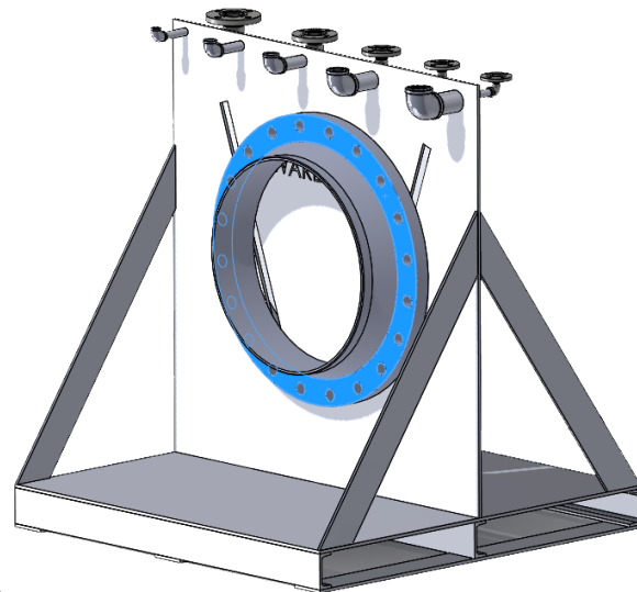
PSV-1824 (18" - 24") Flanges & Valves
