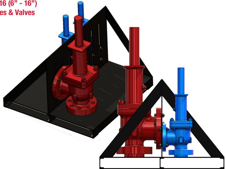
PSV-616 Shown with 6" & 10" Valves Mounted to Rack Frame
