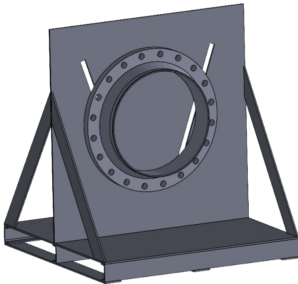
PSV-1824 (18" - 24") Flanges & Valves
