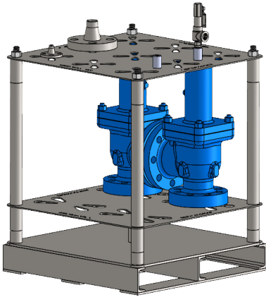
PSV-00504 (6" - 10") Flanges & Valves
