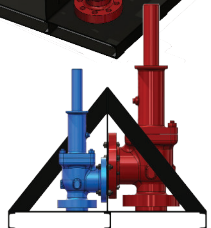
PSV-616 Shown with 6" & 10" Valves Mounted to Rack Frame
