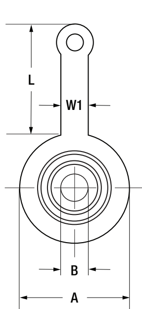
TYPE 2 PADDLE SPACER BLIND
