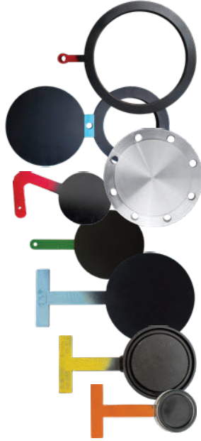
ISOLATION, HYDRO & CUSTOM THICKNESS BLINDS & BLIND FLANGES
